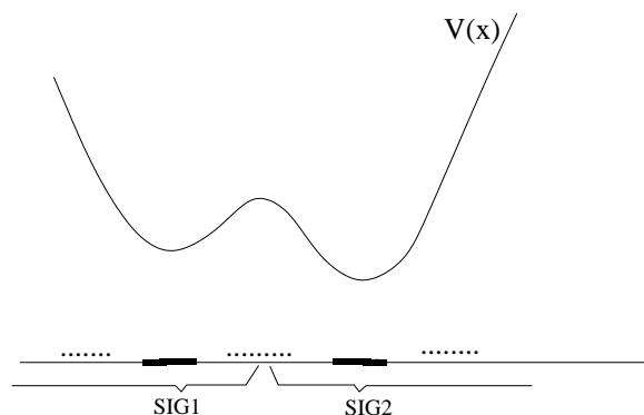
Fig. 5. DSHS for a gradient system
