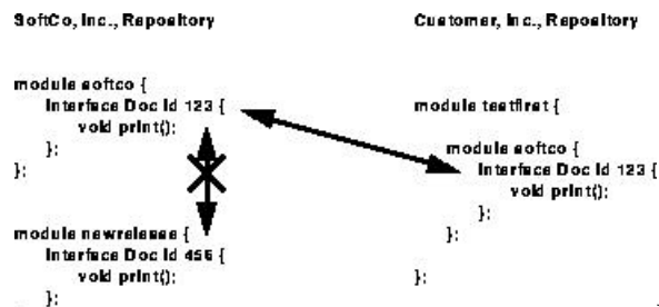
FIGURE 12. Using Repository IDs to establish correspondence between repositories
